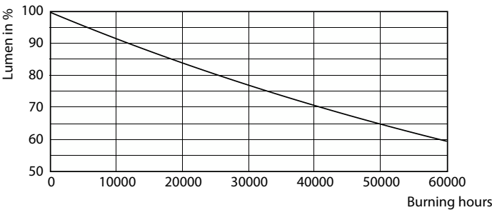
Lumen Maintenance Diagram - MASTER LED 7-50W 927 MR16 24D Dim CN
