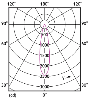
Light Distribution Diagram - MASTER LED 7-50W 927 MR16 24D Dim CN
