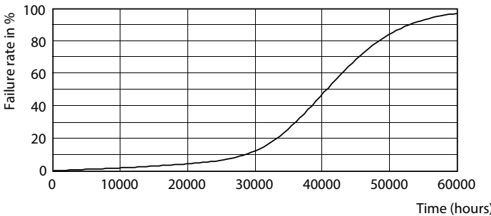
Life Expectancy Diagram - MASTER LED 7-50W 927 MR16 24D Dim CN
