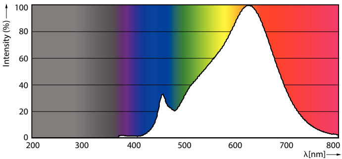
Spectral Power Distribution Colour - MASTER LED 7-50W 927 MR16 36D Dim CN
