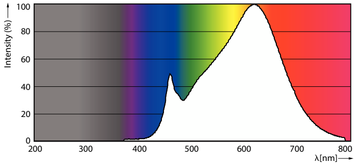
Spectral Power Distribution Colour - MASTER LED 7-50W 930 MR16 36D Dim CN
