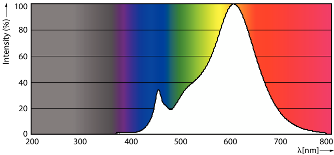
Spectral Power Distribution Colour - MASTER LED 8-50W+ 827 MR16 24D Dim CN
