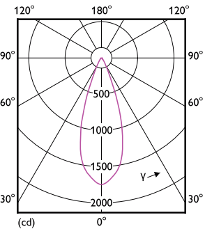
Light Distribution Diagram - 8.5MR16/LED/827/F35/DIM 12V 10/1FB
