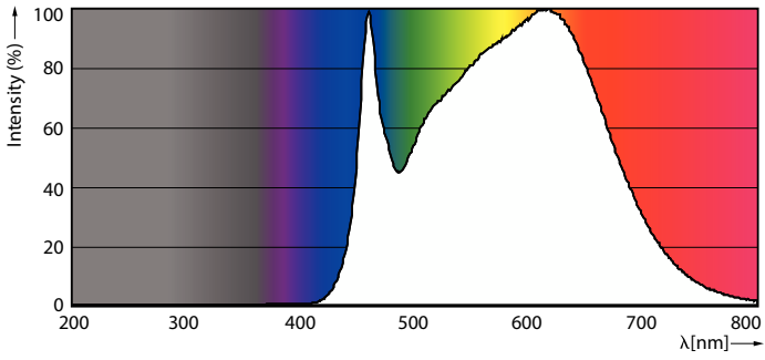
Spectral Power Distribution Colour - MASTER LED 6.5-50W 940 MR16 24D CN
