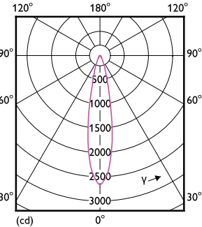
Light Distribution Diagram - MASTER LED 6.5-50W 940 MR16 24D CN
