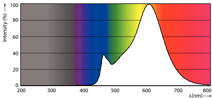
LEDBulb CLA 12-100W E27 A67 CL 827 DIM
