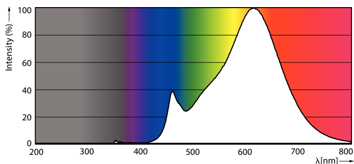
Spectral Power Distribution Colour - LEDClassic SSW 40W B35 E14 WW CL ND 1SRT
