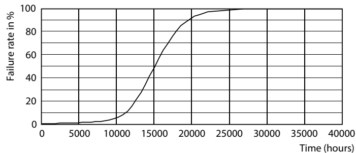
Life Expectancy Diagram - CLA LEDBulb ND 11-100W E27 840 A67 CL
