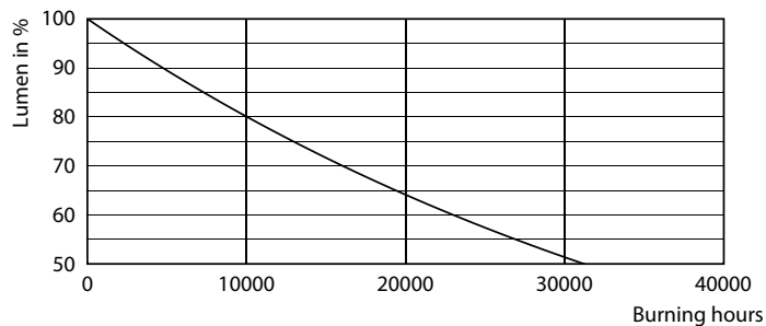
Lumen Maintenance Diagram - CLA LEDBulb ND 11-100W E27 840 A67 CL
