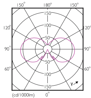
Light Distribution Diagram - CLA LEDCandle ND 4.3-40W E14 827 B35 CL
