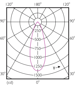
Light Distribution Diagram - Corepro LEDspot 730lm GU10 840 60D
