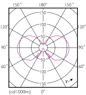
Light Distribution Diagram - CLA LEDBulb D 5.5-40W ST64 E27 827 CL
