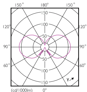
Light Distribution Diagram - CLA LEDCandle D 5-32W BA35 E14 822 GOLD
