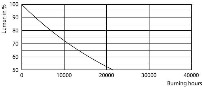
Lumen Maintenance Diagram - LEDBulb 27W E27 6500K 230V A80 APR
