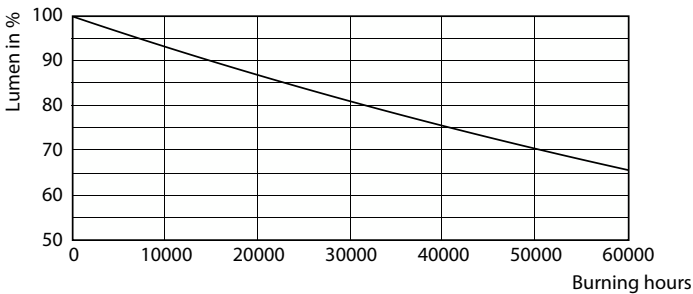
Lumen Maintenance Diagram - TForce LED HPL ND 42-33W E27 730 FR
