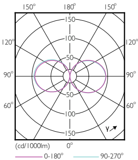
Light Distribution Diagram - TForce LED HPL ND 42-33W E27 730 FR
