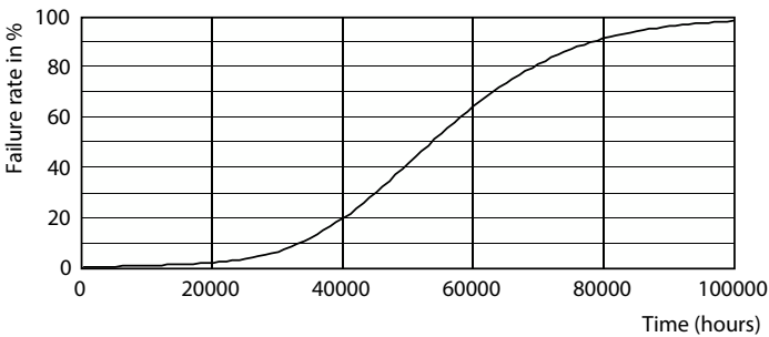
Life Expectancy Diagram - TForce LED HPL ND 42-33W E27 730 FR
