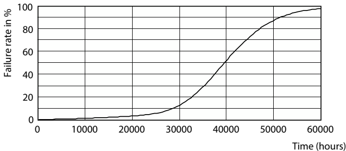
Life Expectancy Diagram - TForce LED HPL ND 42-33W E27 730 FR
