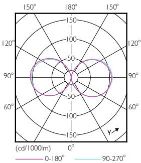
Light Distribution Diagram - TForce LED HPL ND 48-33W E27 740 CL
