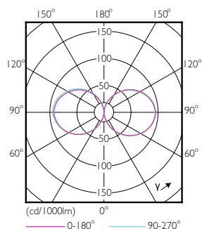
Light Distribution Diagram - TForce LED HPL ND 44-33W E27 740 FR
