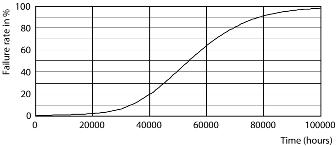
Life Expectancy Diagram - TForce LED HPL ND 44-33W E27 740 FR
