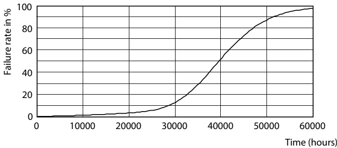
Life Expectancy Diagram - TForce LED HPL ND 28-25W E27 730 FR
