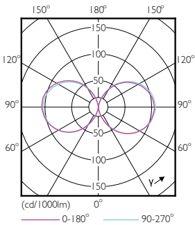
Light Distribution Diagram - TForce LED HPL ND 32-25W E27 740 CL
