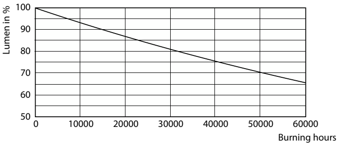
Lumen Maintenance Diagram - TForce LED HPL ND 32-25W E27 740 CL
