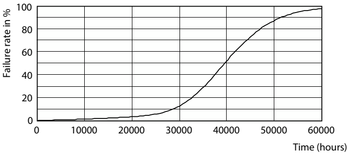
Life Expectancy Diagram - TForce LED HPL ND 32-25W E27 740 CL
