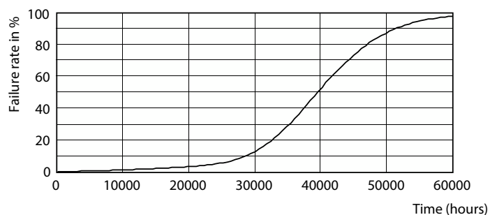
Life Expectancy Diagram - TForce LED HPL ND 29-25W E27 740 FR
