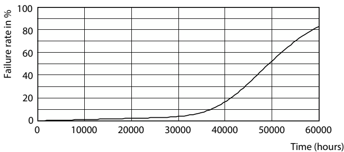
Life Expectancy Diagram - TForce LED Road 55-35W E27 730
