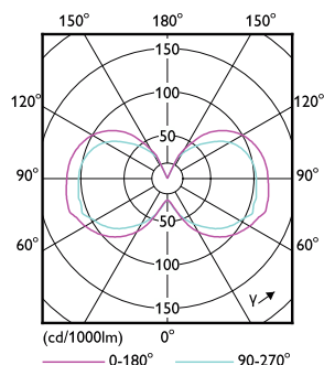
Light Distribution Diagram - CorePro LEDcapsule ND 3.2-40W G9 827
