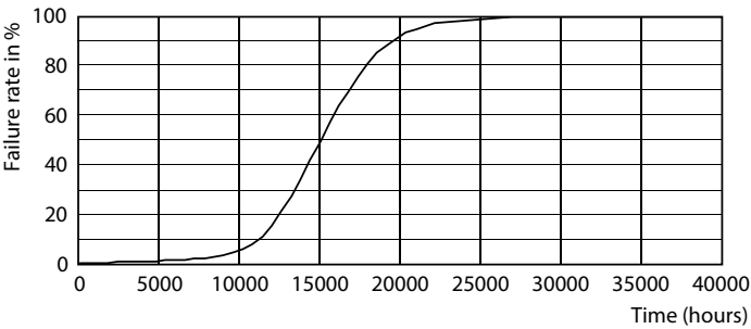
Life Expectancy Diagram - LED giant 25W E27 A160 4000K smoky D
