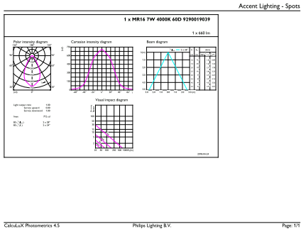
Accent Lighting Spots - MAS LED SPOT VLE D 7-50W MR16 840 60D
