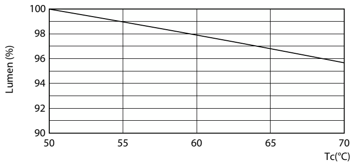
Lumen Maintenance Diagram - MAS LEDtube 1200mm UO 16W 830 T8 FF RCA
