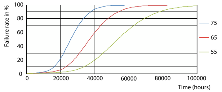
Life Expectancy Diagram - MAS LEDtube 1200mm UO 16W 830 T8 FF RCA
