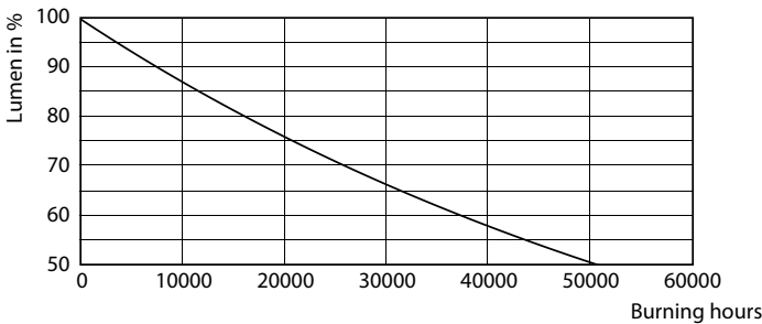
Lumen Maintenance Diagram - 25.5PAR30L/PER/830/F25/ND/120-277V 6/1FB
