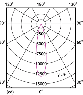
Light Distribution Diagram - 25.5PAR30L/PER/830/F25/ND/120-277V 6/1FB
