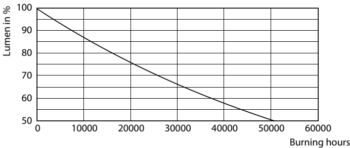
Lumen Maintenance Diagram - 25.5PAR30L/PER/930/F25/ND/120-277V 6/1FB
