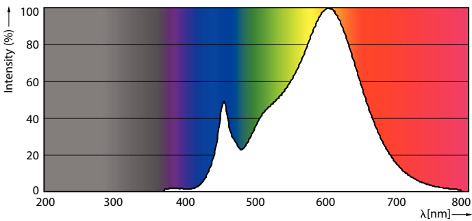
Spectral Power Distribution Colour - 25.5PAR30L/PER/930/F25/ND/120-277V 6/1FB
