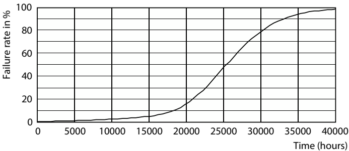
Life Expectancy Diagram - 25.5PAR30L/PER/930/F25/ND/120-277V 6/1FB
