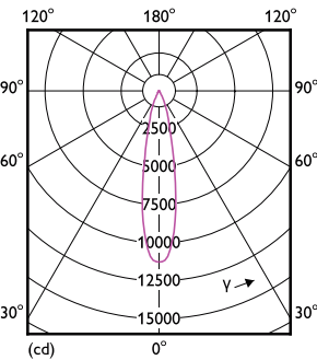
Light Distribution Diagram - 25.5PAR30L/PER/930/F25/ND/120-277V 6/1FB
