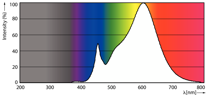
Spectral Power Distribution Colour - 23PAR30s/PER/930/S15/ND/120V 6/1FB
