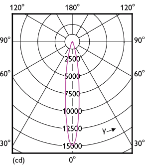
Light Distribution Diagram - 23PAR30s/PER/930/S15/ND/120V 6/1FB
