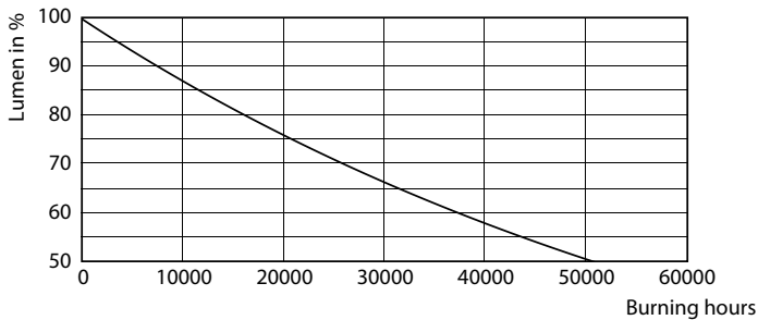
Lumen Maintenance Diagram - 23PAR30s/PER/930/S15/ND/120V 6/1FB
