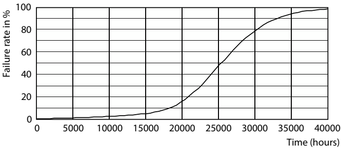
Life Expectancy Diagram - 23PAR30s/PER/930/S15/ND/120V 6/1FB
