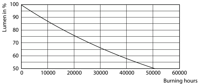
Lumen Maintenance Diagram - 23PAR30s/PER/930/F25/ND/120V 6/1FB
