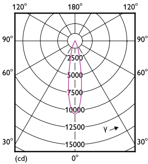
Light Distribution Diagram - 33PAR38/PER/830/F25/DIM/120V B 6/1FB
