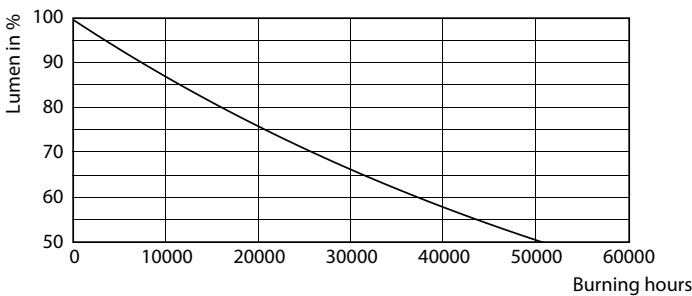
Lumen Maintenance Diagram - 33PAR38/PER/830/F25/DIM/120V B 6/1FB
