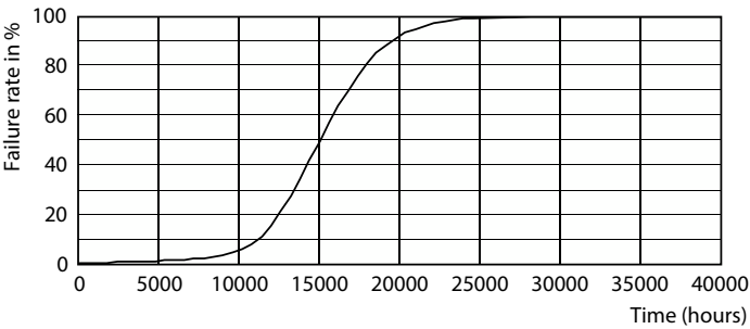
Life Expectancy Diagram - CLA LEDBulb D 8-50W A60 E27 822 GOLD
