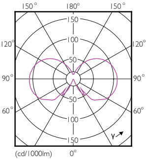
Light Distribution Diagram - CLA LEDBulb D 8-50W A60 E27 822 GOLD
