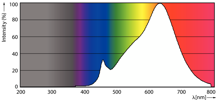
Spectral Power Distribution Colour - 8.5PAR20/PER/927/F25/DIM/EC/120V 6/1FB
