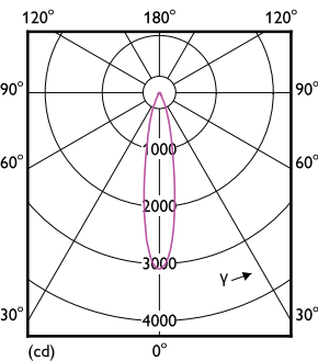
Light Distribution Diagram - 8.5PAR20/PER/927/F25/DIM/EC/120V 6/1FB
