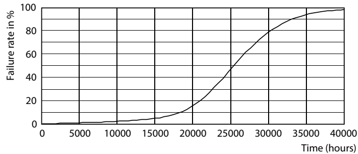
Life Expectancy Diagram - 8.5PAR20/PER/927/F25/DIM/EC/120V 6/1FB
