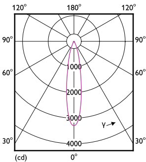
Light Distribution Diagram - 8.5PAR20/PER/940/F25/DIM/EC/120V 6/1FB
