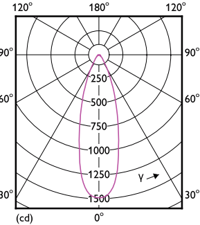
Light Distribution Diagram - 8.5PAR20/PER/930/F40/DIM/EC/120V 6/1FB
