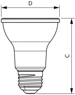
PAR20 120V 9-50W 560lm 40D 3000K E26 D
