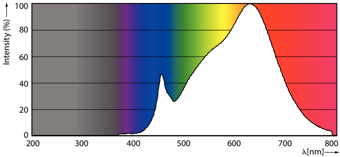
Spectral Power Distribution Colour - 8.5PAR20/PER/930/F40/DIM/EC/120V 6/1FB
