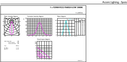
Light Distribution Diagram - 8.5PAR20/PER/930/F40/DIM/EC/120V 6/1FB
