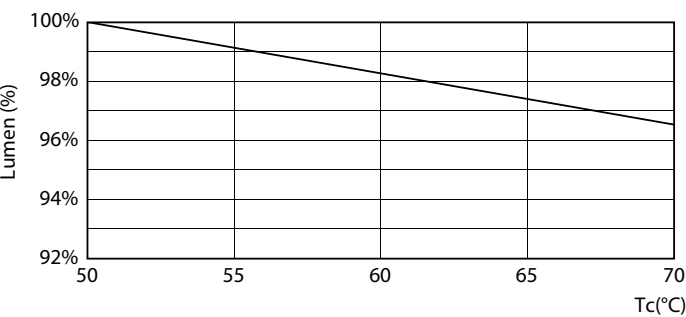
Lumen Maintenance Diagram - MAS LEDtube 1200mm HO 12.5W 865 T8
