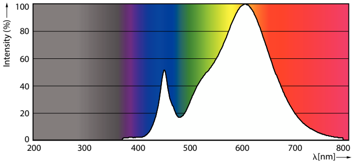
Spectral Power Distribution Colour - TForce Core LED PT 50-42W E27 830 FR
