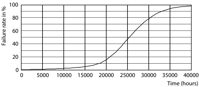
Life Expectancy Diagram - TForce Core LED PT 50-42W E27 830 FR
