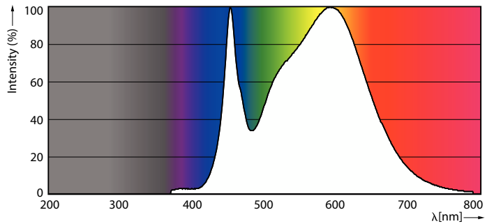
Spectral Power Distribution Colour - TForce Core LED PT 50-42W E27 840 FR
