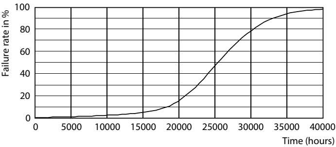
Life Expectancy Diagram - TForce Core LED PT 50-42W E27 840 RCA
