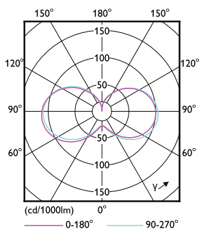
Light Distribution Diagram - TForce Core LED PT 30-27W E27 840 FR
