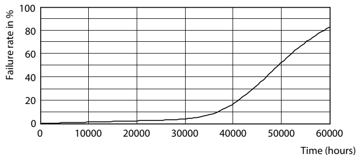
Life Expectancy Diagram - TForce LED HB MV ND 120-100W E40 840 NB
