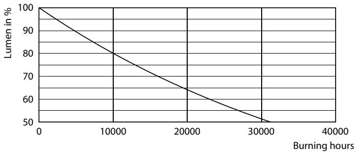
Lumen Maintenance Diagram - 5A19/PER/822-827/E26/CL/G/WGX 10/1CT
