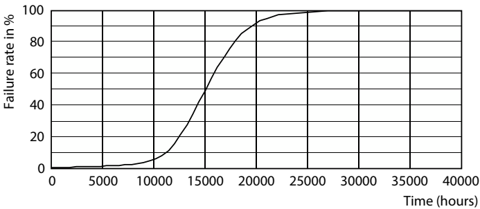
Life Expectancy Diagram - 5A19/PER/822-827/E26/CL/G/WGX 10/1CT
