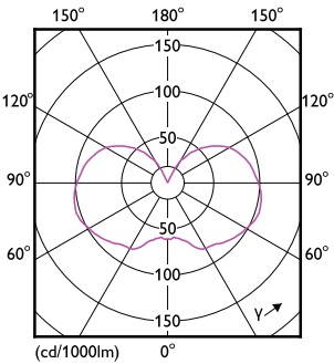
Light Distribution Diagram - 5A19/PER/822-827/E26/CL/G/WGX 10/1CT
