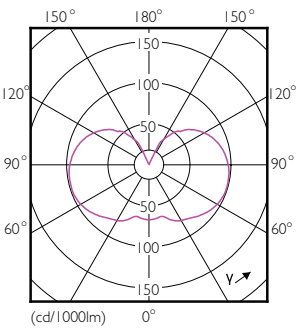
Light Distribution Diagram - 4G25/PER/822-827/E26/CL/G/WGX 10/1CT
