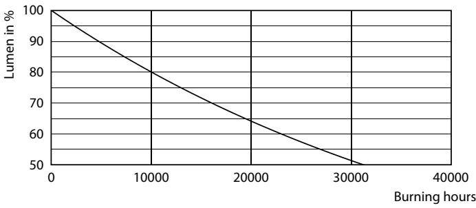
Lumen Maintenance Diagram - 4G25/PER/822-827/E26/CL/G/WGX 10/1CT
