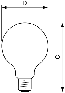
Bulb G93 8-50W 630lm 2200K E27 D Amber
