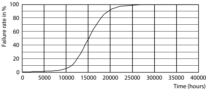
Life Expectancy Diagram - LEDClassic 12W Heart E27 2000K GOLD ND
