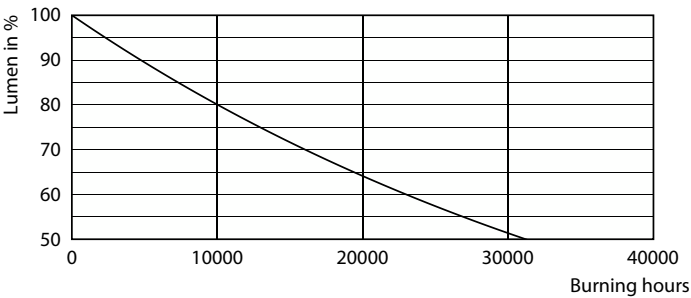
Lumen Maintenance Diagram - LEDClassic 12W Heart E27 2000K GOLD ND
