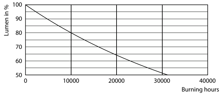
Lumen Maintenance Diagram - 7.5A50/modern/840/CL/G/DIM 2/1CT
