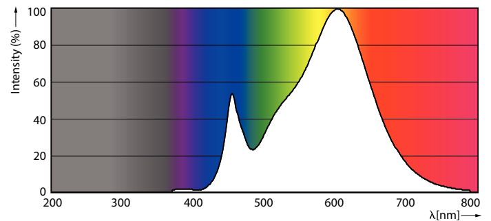
Spectral Power Distribution Colour - TForce Core HB MV ND 26-24W E27 830
