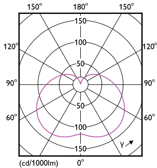
Light Distribution Diagram - TForce Core HB MV ND 26-24W E27 830
