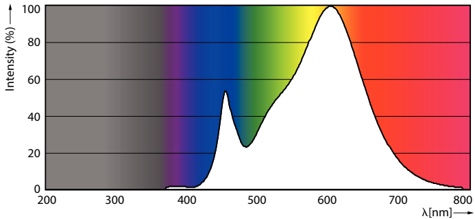
Spectral Power Distribution Colour - TForce Core HB MV ND 48-42W E27 830
