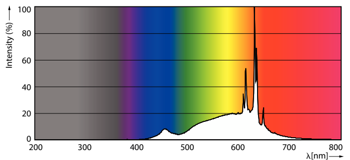
Spectral Power Distribution Colour - 5A19/MAS/927-22/FR/P/E26/T20 6/1CT
