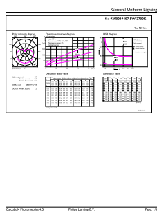
General uniform lighting - 5A19/MAS/927-22/FR/P/E26/T20 6/1CT
