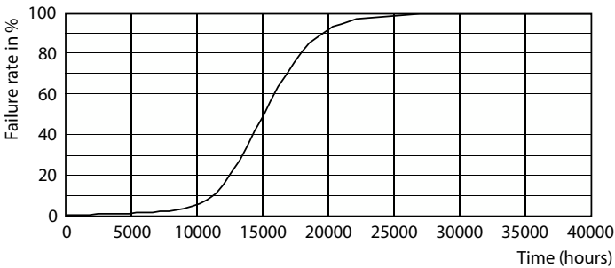
Life Expectancy Diagram - LEDClassic 48W A60 E27 825 100-240V NDLA
