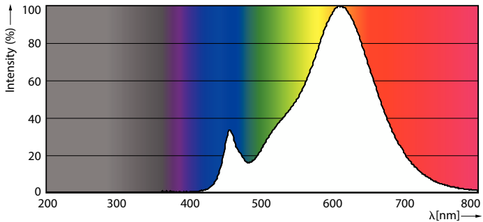
Spectral Power Distribution Colour - LEDClassic 48W A60 E27 825 100-240V NDLA
