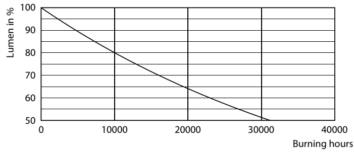
Lumen Maintenance Diagram - LEDClassic 48W A60 E27 825 100-240V NDLA
