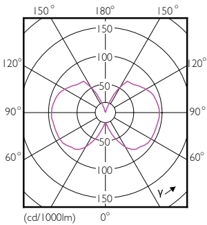
Light Distribution Diagram - LEDClassic 48W A60 E27 825 100-240V NDLA
